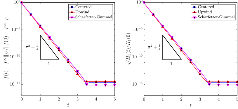
FIGURE 2. Decay to the steady state associated to each scheme in L^1 norm (left) and Boltzmann entropy (right) for each scheme. Here the mesh is that of Figure 1 ( \Delta x = 1/4 ). Time step: \Delta t = 10^{-2} .
