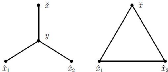
FIGURE 7. Star-triangle transformation.
