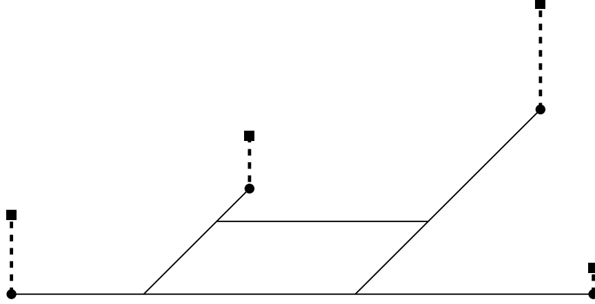
FIGURE 2. Sketch of a graph and positive boundary conditions at the four boundary points in A . This is a picture in dimension 2 + 1 , and dashed lines and squares represent the height of the boundary conditions.
