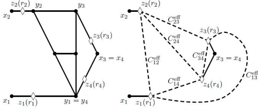
FIGURE 6. The original network \tilde{\mathcal{G}} on the left and the network after rewiring on the right. Dashed lines are the edges used for rewiring, with corresponding effective conductances.
