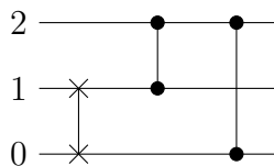
Figure 8. Simplification of the circuit of figure 7.
