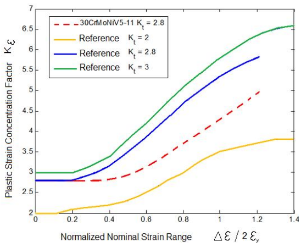
Figure 4. Strain Concentration Factor
