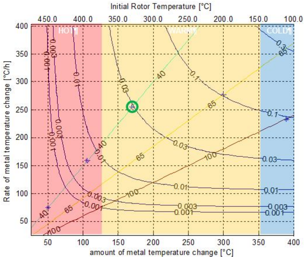
Figure 9. Cyclic Life Expenditure curves for the High Pressure part of the Rotor (blue curves); experimental start up data (blue stars); result about the Warm Start Up of Table 3 (green circle); minutes to full temperature (colored straight lines).
