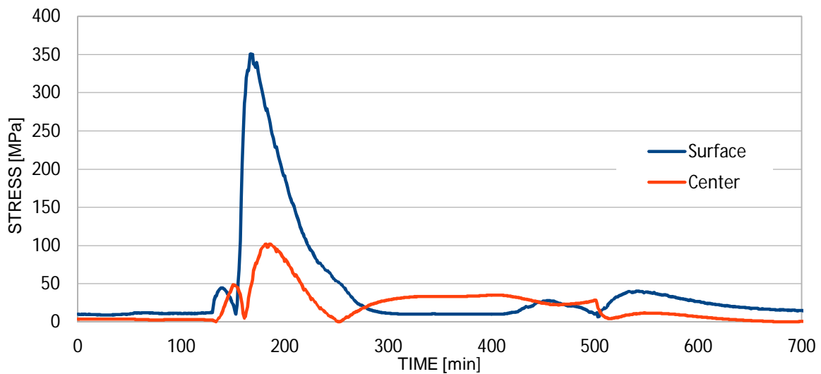
Figure 8. Von Mises Equivalent Stress
