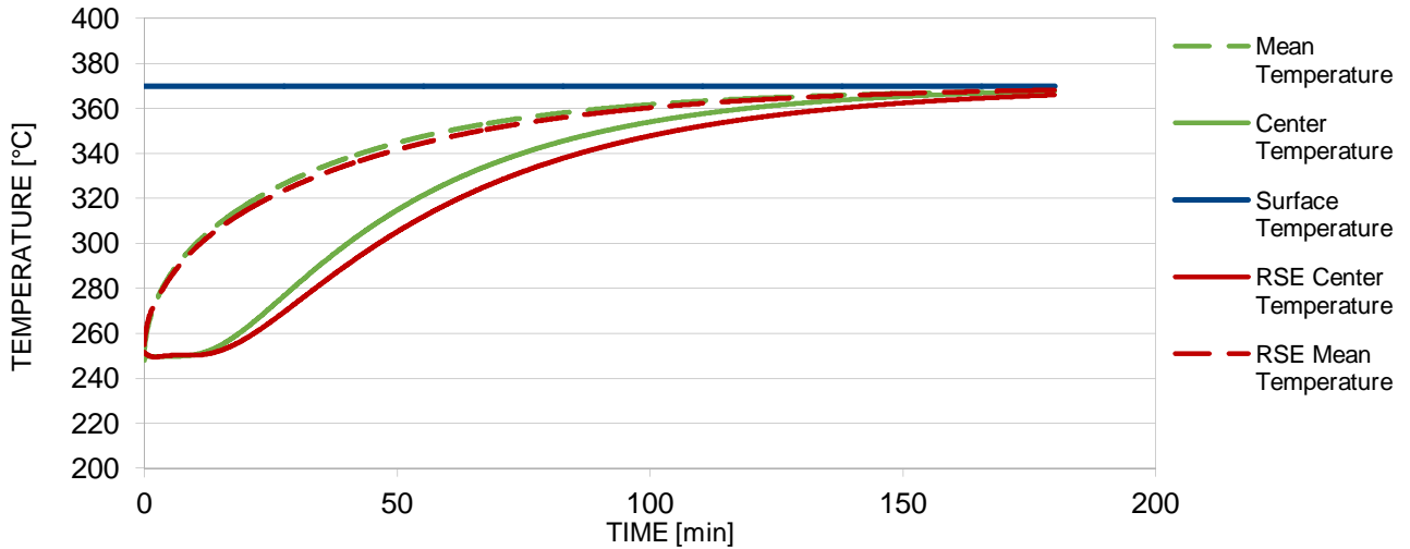
Figure 2. Temperature Comparison for a step change in the surface temperature
