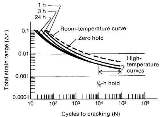
Figure 5. Low Cycle Fatigue Curves for Cr-Mo-V Rotor Steels at Approximately 540°C [5]
