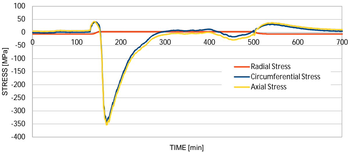
Figure 7. Surface - Radial, Circumferential and Axial Stresses
