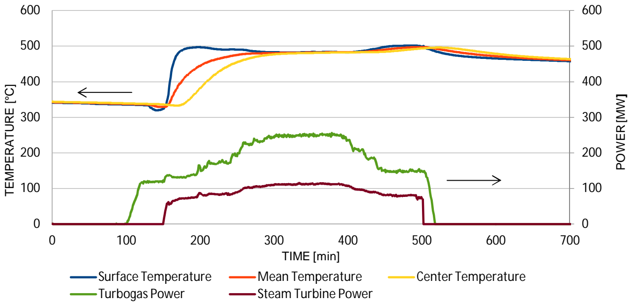
Figure 6. Temperatures and Powers
