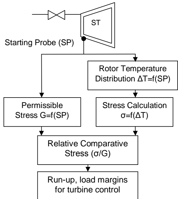
Figure 1. Rotor Stress Evaluator Calculation Scheme
