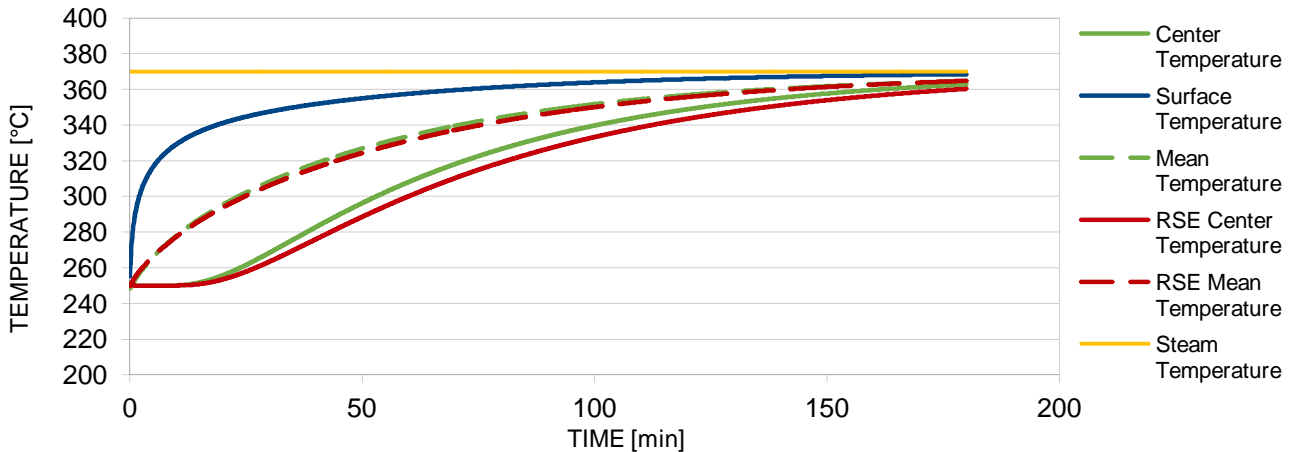
Figure 3. Temperature Comparison for a step change in the steam temperature
