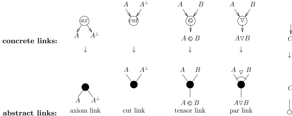
Fig. 2. transforming concrete proof structures into abstract proof structures
