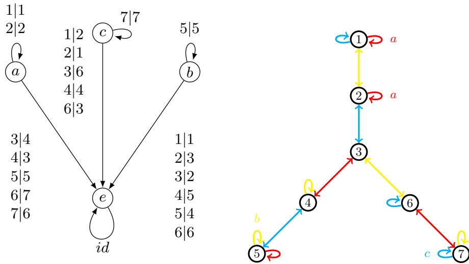
Figure 9: A novel automata generating a group of intermediate growth (on the left) and its Schreier graph on level 1 (on the right).
