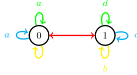
Figure 2: The automata generating the first Grigorchuk group.
