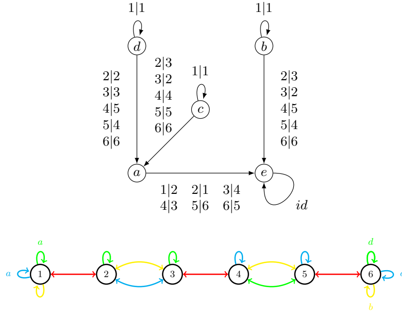
Figure 7: A novel automata generating a group of intermediate growth (on the top) and its Schreier graph on level 1 (on the bottom). Notice the similarities with the Grigorchuk group on Fig. 2.
