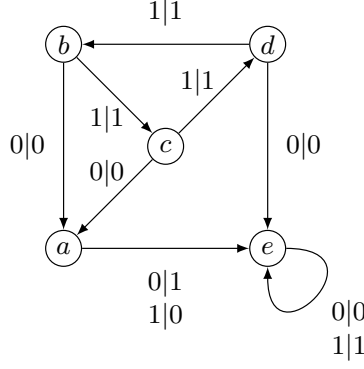
Figure 2: The automata generating the first Grigorchuk group.
