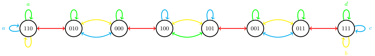
Figure 5: The automata generating the first Grigorchuk group on level 3.
