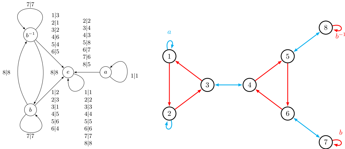
Figure 8: The automaton a = \langle a, e, e, e, e, e, e, e \rangle(3, 4)(5, 8)(6, 7) ; b = \langle e, e, e, e, e, e, b, b^{-1} \rangle(1, 2, 3)(4, 5, 6) (on the left) from [16] and its Schreier graph on level 1 (on the right).
