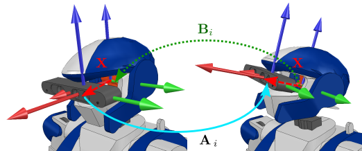
Fig. 2. Hand-Eye Calibration : the relative camera motion \mathbf{A}_i and the relative robot motion \mathbf{B}_i and the unknown extrinsic transformation \mathbf{X} are forming a closed kinematic loop.
