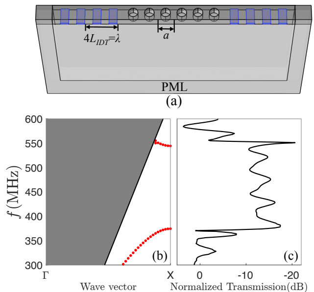
FIG. 5: (a) Schematic of the SAW device model for calculating the transmission spectra of Love waves through the PnC. r = 0.3a , H = 0.6a , a = 4\mu\text{m} ; (b) Zoom of the band structure of Love modes around the band-gap zone in the \Gamma -X direction; (c) Normalized transmission spectra of Love waves propagating through the PnC around the band-gap zone. N_{PnC} = 10 , N_{IDT} = 20 , h_{IDT} = 200\text{nm} , V_0 = 1\text{V} .
