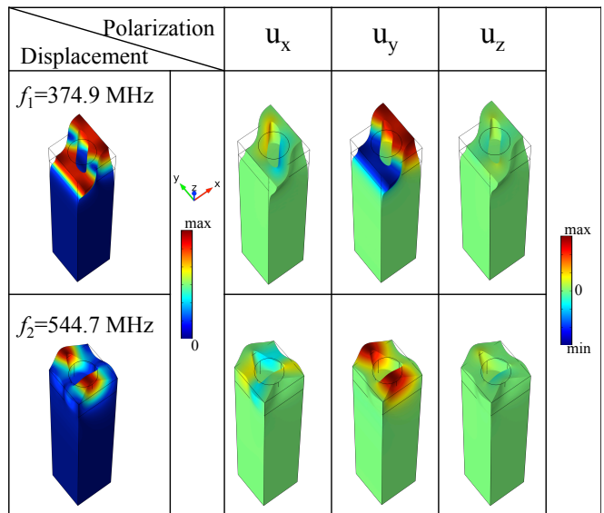
FIG. 4: Displacement fields and polarizations of the two Love modes at 374.9 and 544.7 MHz. r = 0.3a , H = 0.6a , a = 4\mu\text{m} .
