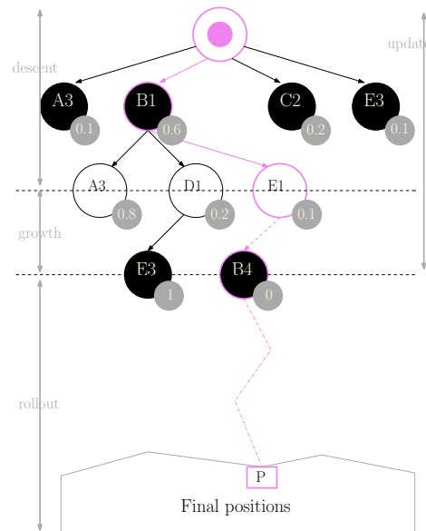
Fig. 5. The four stages of the MCTS algorithm
