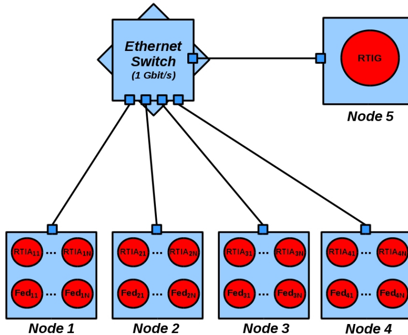
Figure 6. Deployment of CERTI federation over classical Ethernet architecture
