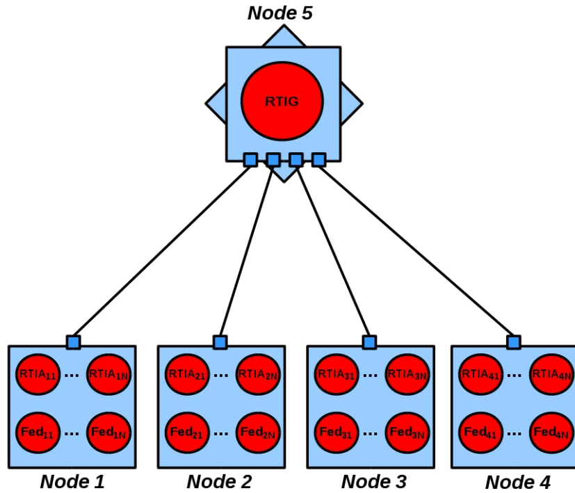
Figure 7. Deployment of CERTI federation over classical Ethernet architecture
