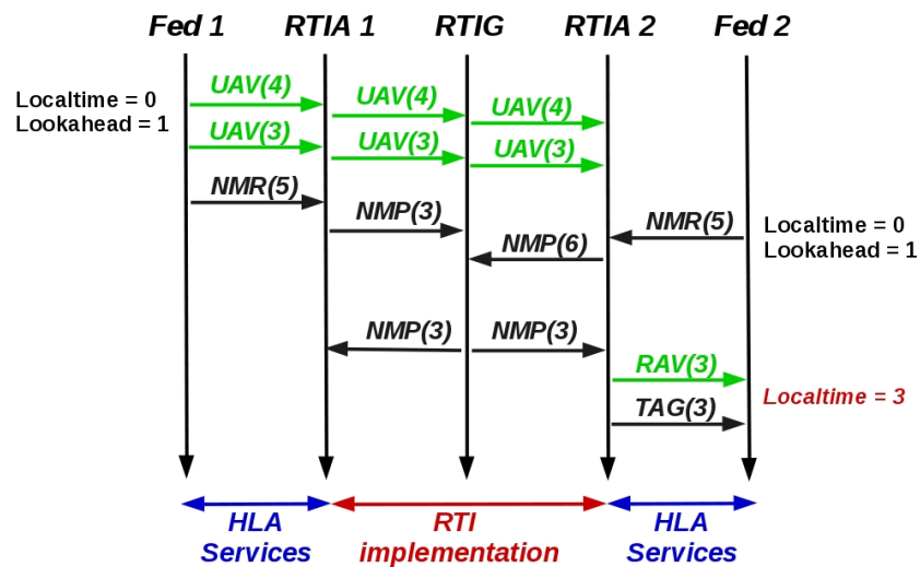
Figure 5. UAV/NMR/TAG message exchanges illustration for NMP protocol (event-driven federates)
