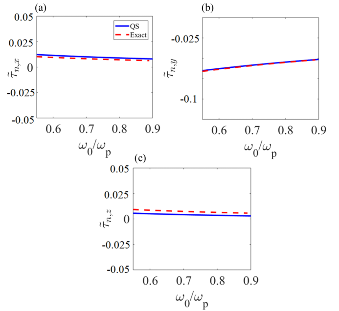
FIG. 5. Nonresonant part of the optical torque (fluctuation-induced Casimir torque) on an atom in its ground state, with \gamma = (1 + i)\hat{x} + i\hat{y} + \hat{z} , sweeping the radiation frequency in the range [\omega_-, \omega_+] (the other parameters of the system are given in the caption of Fig. 3). The three panels show the three Cartesian components of the torque, comparing the quasistatic solution (solid blue) with the exact solution (dashed red).
