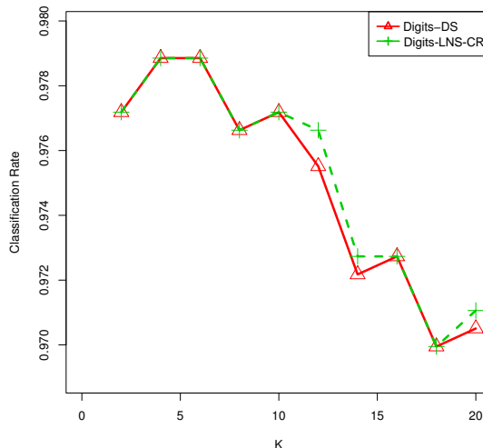
Fig. 16. Classification rates on Digits data set.
