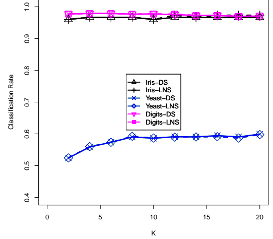
Fig. 15. Classification results with different values of K on UCI data set. In the figure, the legend “Iris-DS” means it is the classification rates on Iris data set using DS combination rule. Same as the other legends.
