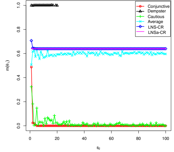
Fig. 9. The mass on \{\theta_1\} after the combination with s_2 ranging from [0,100] and s_1 = 4 * s_2 .
