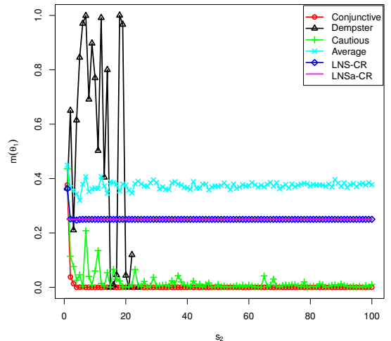
Fig. 6. The mass on \{\theta_1\} after the combination with s_2 ranging from [0, 100] and s_1 = s_2 .
