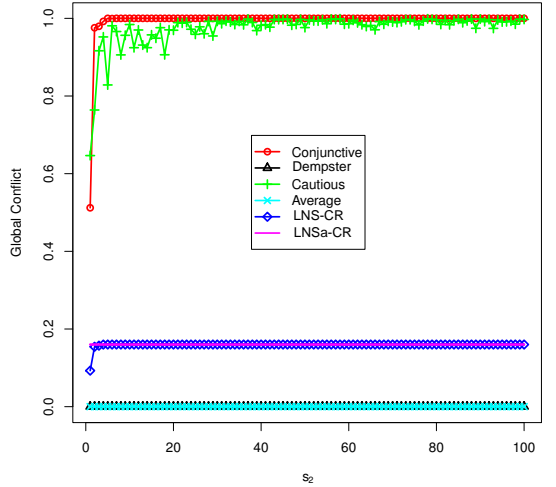
Fig. 5. The global conflict after the combination with s_2 ranging from [0, 100] and s_1 = 4 * s_2 .
