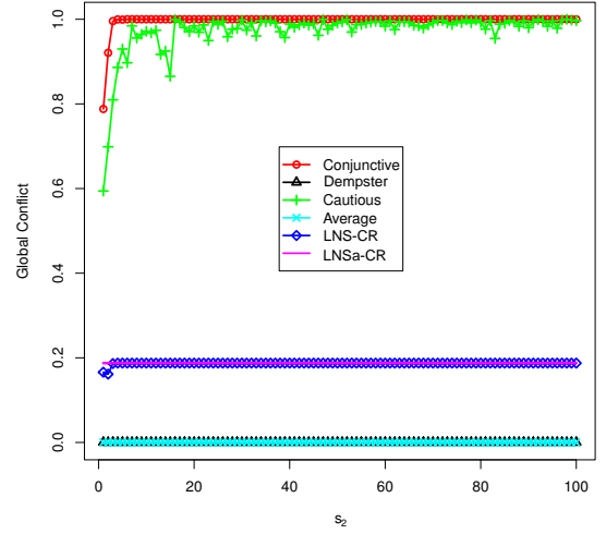
Fig. 4. The global conflict after the combination with s_2 ranging from [0, 100] and s_1 = 3 * s_2 .
