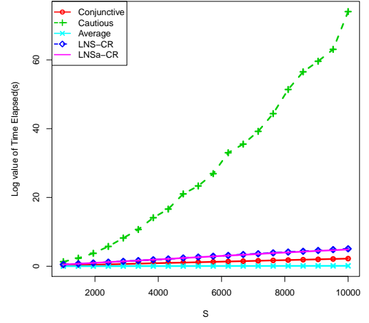
a. Time lapse by five different rules
