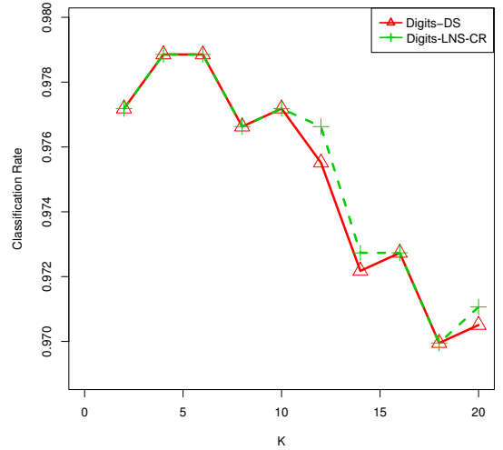
Fig. 16. Classification rates on Digits data set.
