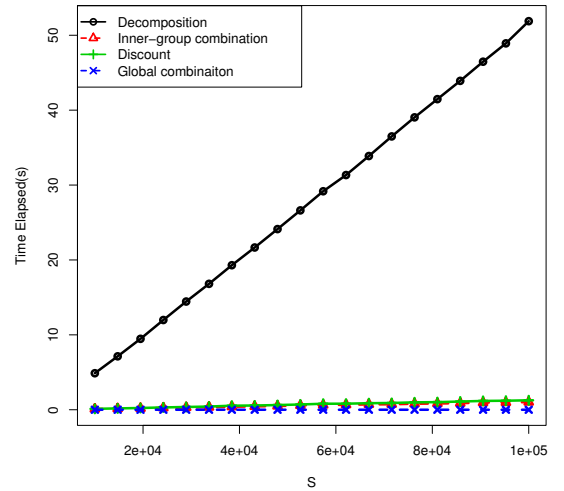
Fig. 12. Time lapse of each step using LNS combination rule with S varying from 10,000 to 100,000.
