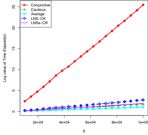
a. Time lapse by five different rules
