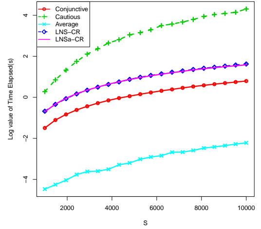
b. The log value of Time lapse by five different rules
