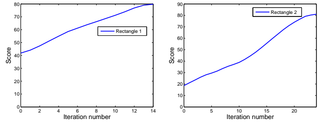
Figure 6: The score evolution as a function of the iteration number associated with the two rectangles shown in Figure 5(c) (the upper left corner). Iteration 0 corresponds to the coarse support and the final iteration corresponds to a local maximum. One can notice that both supports have converged to the same superstructure (see Figure 5(d)).
