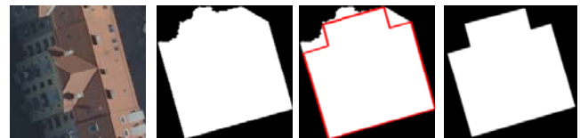
Figure 5: (a) building visible in vertical aerial image (b) segmentation result (c) in red modified building outline using 3D façade reconstruction (d) enhanced building footprint.
