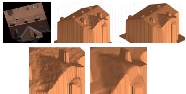
Figure 2: (a) Shows RGB image of single building of our test dataset (b) shows range image without using TGV model (c) shows range image using TGV model (d) shows detail of raw range data (e) shows detail of range data using TGV.
