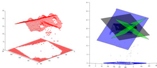
Figure 3: (left) Axonometric view of smoothed 3D point cloud of building roof (GSD 10cm) (points are highlighted in red); Dimensions: x,y-axis [in pixels], z-axis [in m] (right) 3D Point cloud of roof highlighted in blue; overlaid are the two major planes, marked in blue and the two smaller planes in green.
