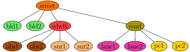
Figure 3: An example DAG-structured object hierarchy: sdwlc(sidewalk), bld(building), sur(surface), pc(pedestrian crossings, obs(obstacle))
