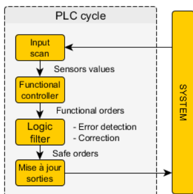
Figure 1: Principle of the logic filter.
