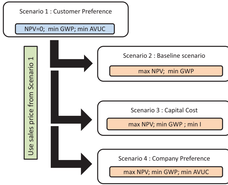
Fig. 4. Sequential optimization scheme.
