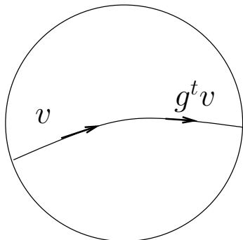
Figure 2: Geodesic flow
