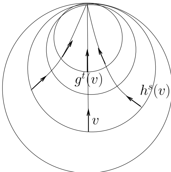
Figure 3: Horocyclic flow
