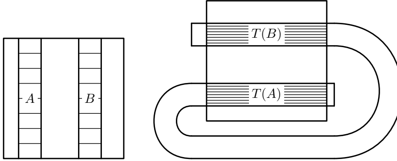
FIGURE 8. Smale's horseshoe
