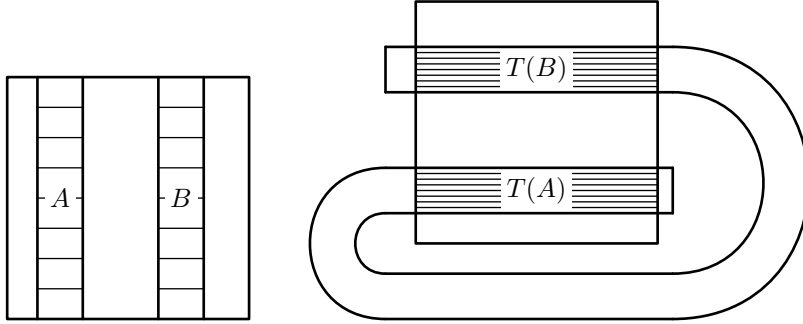
FIGURE 8. Smale's horseshoe
