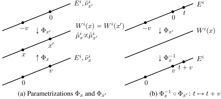
FIGURE 2. Proof of Lemma 6.3
