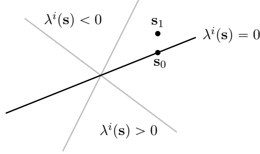
FIGURE 3. Choice of s_1
