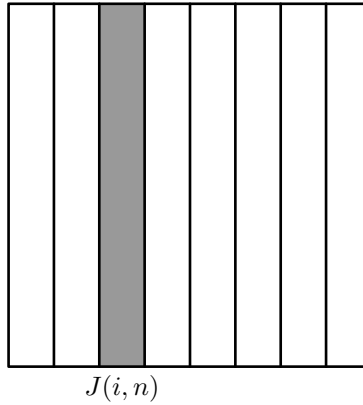
FIGURE 5. A measurable partition of \mathbb{T}^2 .
