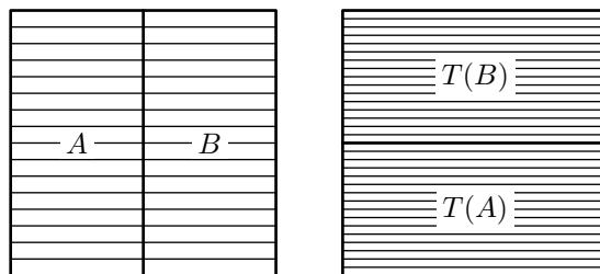
FIGURE 7. The baker transformation
