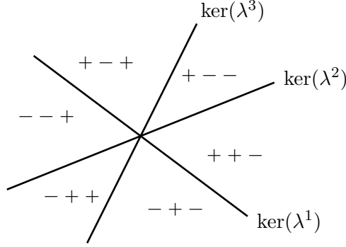
FIGURE 1. Kernels of the Lyapunov exponent functionals in the acting group \mathbb{R}^2 . Signs indicate the signs of the Lyapunov exponents in corresponding half-cones. For instance, ++- indicates the open half-cone of s \in \mathbb{R}^2 such that \lambda^1(s) > 0 , \lambda^2(s) > 0 , and \lambda^3(s) < 0 .
