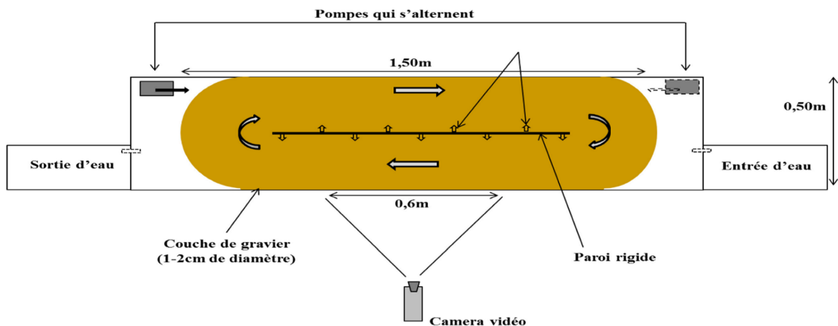
Figure 1 - Diagram of the aquarium [10]
