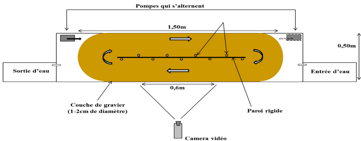
Figure 1 - Diagram of the aquarium [10]
