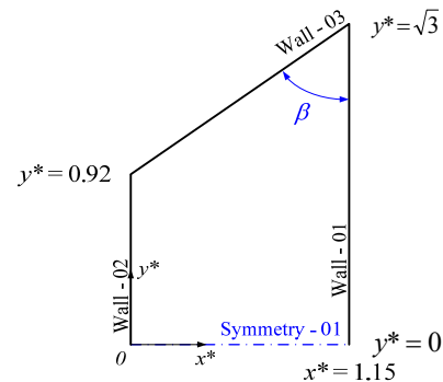
Figure 7b: trapezoidal section with D_h^* = 1.502 ; \beta = 54.74^\circ
