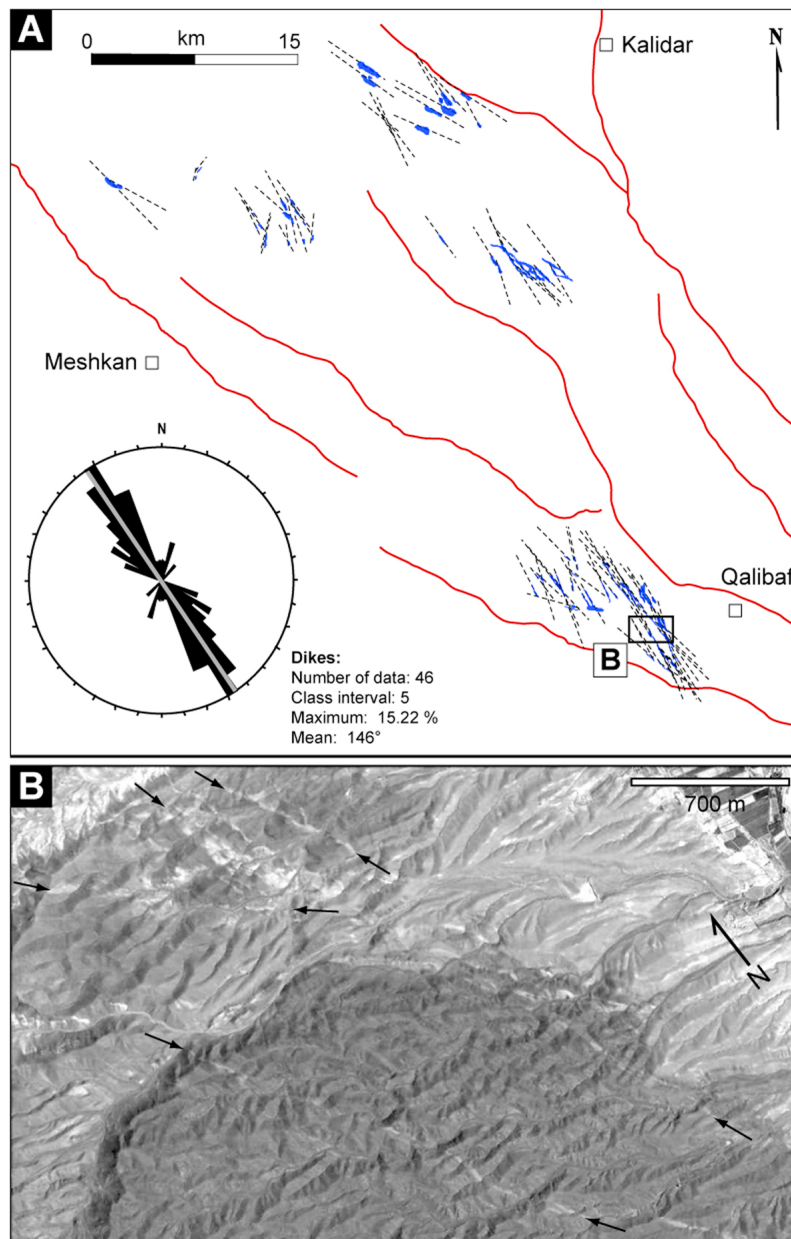
Figure 3. (a) Map of Miocene-Pliocene dikes (blue closed polygons) affecting the southeastern part of the Meshkan area. Dashed lines indicate orientation of dikes. Preferred orientation ( \sim N146^{\circ}E ) of the dikes is shown by the lower left rose diagram. (b) QuickBird image (Google Earth), showing dikes intruded the Eocene-Oligocene rocks in the southeast of the Meshkan area (see Figure 3a for the location).
