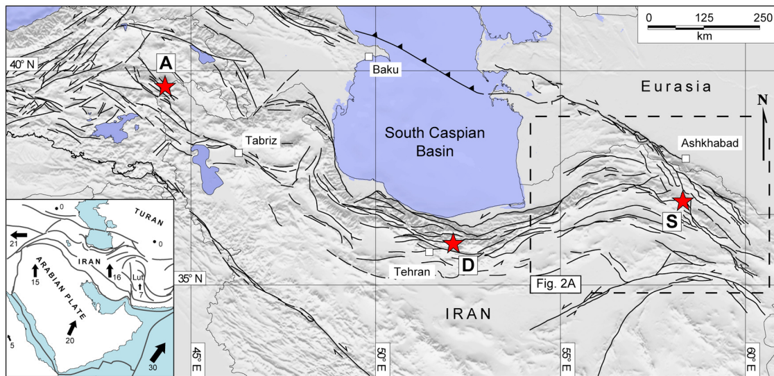
Figure 1. GTOPO30. Shaded relief image showing the location of Sar'akhor (S), Damavand (D), and Ararat (A) volcanoes in the northern part of the Arabia-Eurasia collision zone. Fault traces (black line) are after Bozkurt [2001], Koçyigit et al. [2001], Jackson et al. [2002], Hessami et al. [2003], Shabanian et al. [2010], and Solaymani Azad et al. [2011a]. Lower left inset shows the geodynamic setting of Arabia-Eurasia collision/subduction framework. Black arrows and associated numbers (in mm/yr) represent the present-day Arabia-Eurasia plate velocities after Reilinger et al. [2006].
