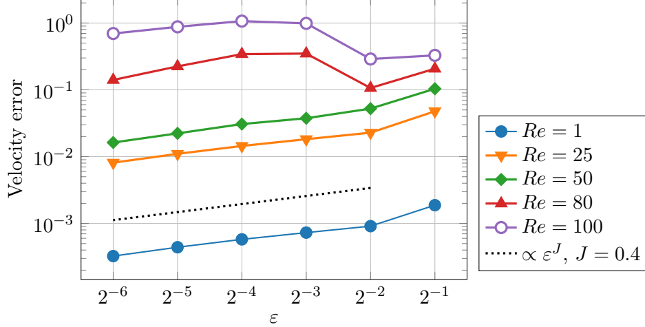
Figure 5: Errors (Eq. (24)) of the Navier-Stokes MAPDD model w.r.t. to the full solution for different Reynolds numbers, with C = 3/\ln(2) ; the line \varepsilon^{J=0.4} for reference.
