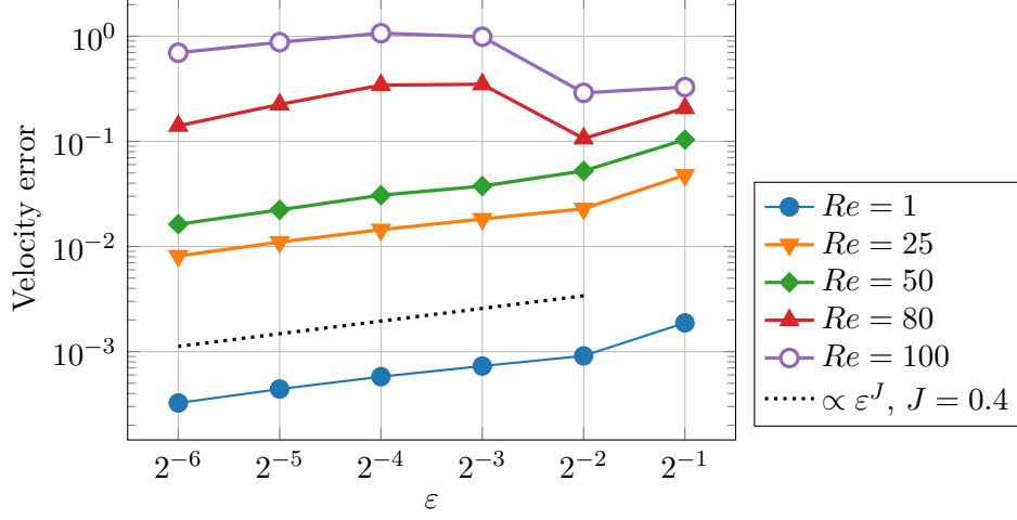
Figure 5: Errors (Eq. (24)) of the Navier-Stokes MAPDD model w.r.t. to the full solution for different Reynolds numbers, with C = 3/\ln(2) ; the line \varepsilon^{J=0.4} for reference.
