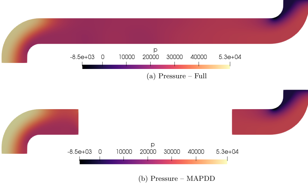
Figure 8: Pressure fields of the transient Navier-Stokes test case at peak time t = 0.2 s, for Re = 2500 , \varepsilon = 0.25 . Full model (a) versus MAPDD model (b).
