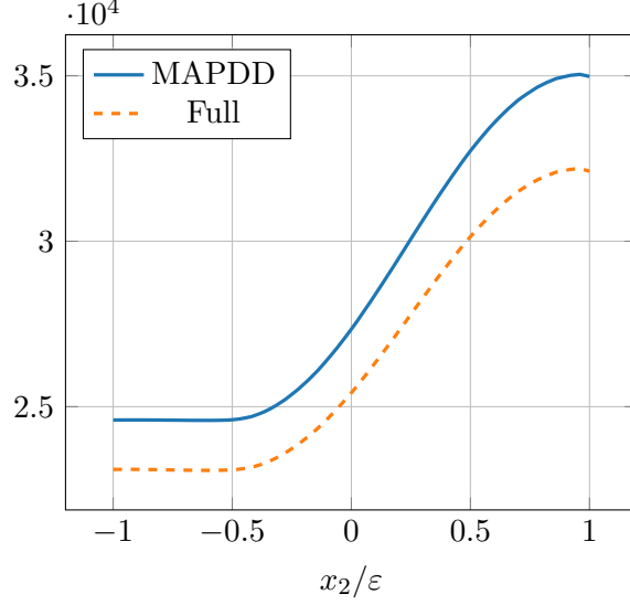
Figure 11: Pressure along the tube cross-section, at 2\varepsilon upstream of \Sigma_1 , for the MAPDD and the full solutions computed for Re = 2500 , \varepsilon = 1/4 .
