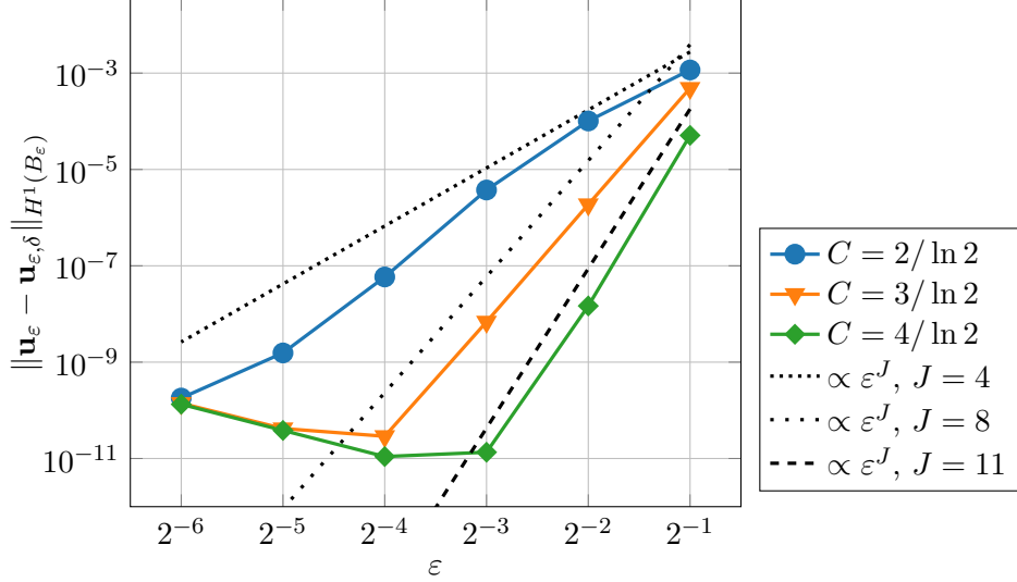
Figure 3: Stationary Stokes test case: convergence of the error with respect to \varepsilon for different values of C (see legend).
