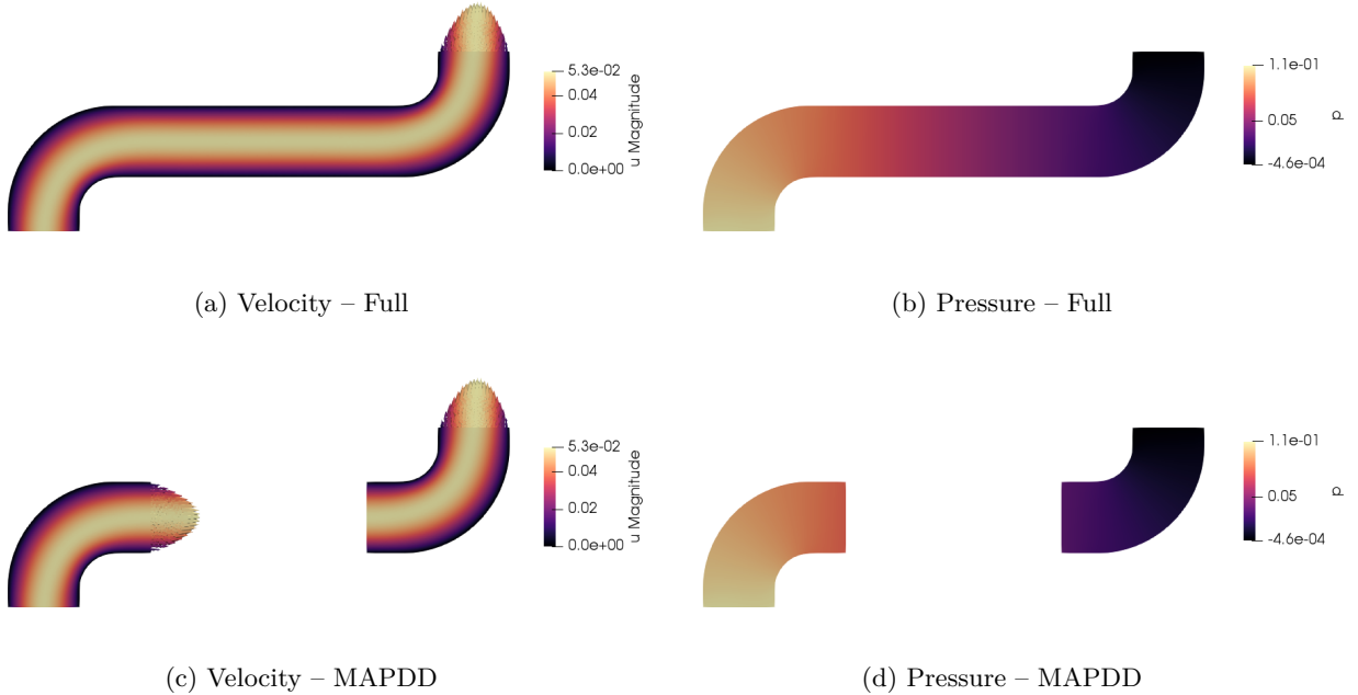
Figure 2: Pressure fields and velocity magnitude and vectors at the outflow boundaries obtained for the stationary Stokes problem using \varepsilon = 0.5 with the full model (top row) and with the MAPDD model (bottom row).
