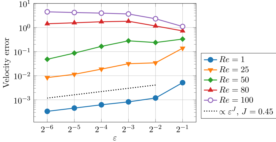
Figure 4: Errors (Eq. (24)) of the Navier-Stokes MAPDD model w.r.t. to the full solution for different Reynolds numbers, with C = 2/\ln(2) ; the line \epsilon^{J=0.45} for reference.
