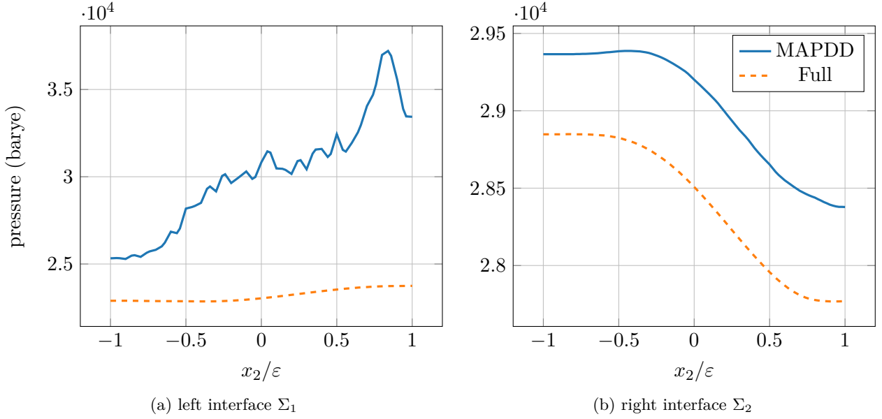
Figure 10: Pressure along the interfaces for the MAPDD and the full solutions computed for Re = 2500 , \varepsilon = 1/4 .
