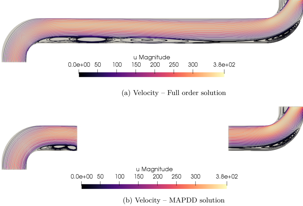
Figure 7: Velocity stream lines of the transient Navier-Stokes test case at peak time t = 0.2 s, for Re = 2500 , \varepsilon = 0.25 . Full model (a) versus MAPDD model (b).
