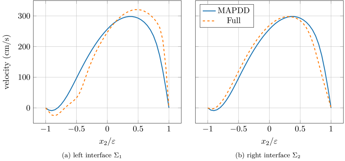
Figure 9: Axial velocity component u_0 at the interfaces for the MAPDD and the full solutions computed for Re = 2500 , \varepsilon = 1/4 .
