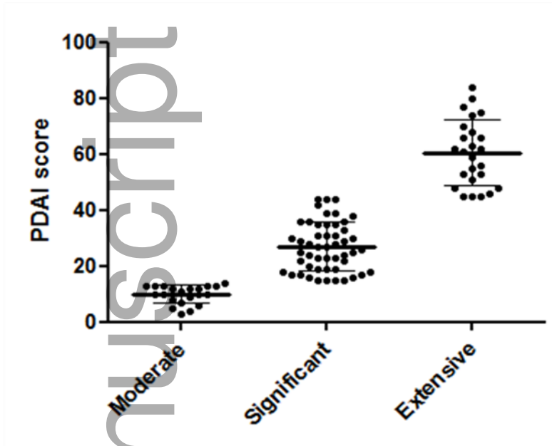
PANEL A: Distribution of PDAI in the 3 subgroups according to PDAI cut-offs
