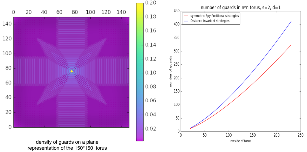
Figure 2: Experimental results, s = 2 and d = 1 . (Left) Density of guards on a plane representation of the 150 \times 150 torus in an optimal symmetrical Spy-positional configuration. (Right) Minimum total amount of guards for symmetrical (red) and distance-invariant (blue) Spy-Positional strategies.
