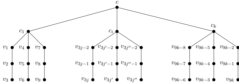
Figure 1: Scheme of the tree T (in the proof of Lemma 3) where only the subtrees S_1, S_i and S_k have been depicted (for some i such that 2 \leq i < k ). In the subtree S_i , \{j, j', j''\} = \{3i - 2, 3i - 1, 3i\} , i.e. , i = \lceil \frac{z}{3} \rceil for every z \in \{j, j', j''\} .
