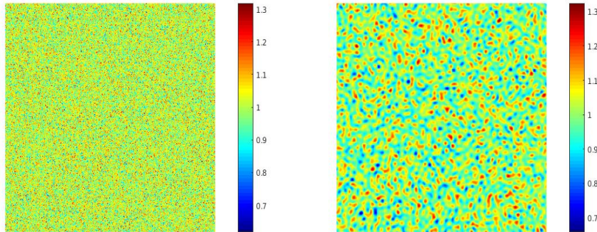
Figure 7: Random media: background (i.e. average value) is one, with mean-zero random perturbations. Left: rough medium close to spatial white noise. Right: smoother medium with larger correlation length. The amplitudes of the fluctuations in both media are similar.
