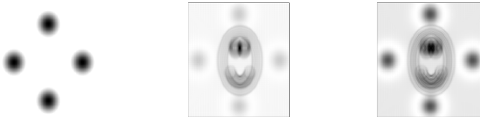
Figure 2: Refocused signal for p_1 as in figure 1 and p_0 given by the function represented on the left panel. Left: initial condition p_0 . Middle: perturbation of duration 13h for a constant function \eta_\tau . Right: perturbation of duration 13h for an uneven function \eta_\tau . The strength of the contribution of p_0 increases when \eta_\tau is not even.
