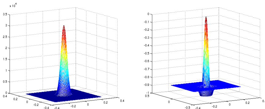
Figure 3: Refocused signal after two perturbations of duration h . Left: a Gaussian initial condition for p_0 . Right: refocused signal at 4T . We verify that the latter is indeed proportional to the laplacian of p_0 .
