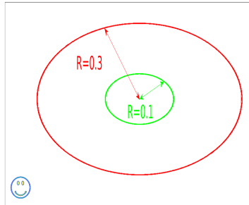
Figure 4: Depiction of the initial condition and the support of the function \chi , which is the smoothed characteristic function of either the small or the large disk where the waves are perturbed.
