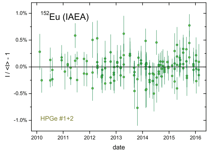
Figure 29. Residuals from exponential decay for ^{152}\text{Eu} activity measurements by \gamma -ray spectrometry with two HPGe detectors at IAEA.
