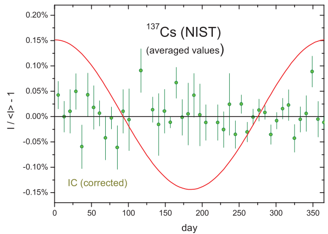
Figure 43. Annual average residuals from exponential decay for ^{137}\text{Cs} activity measurements with IC ‘A’ at NIST.
