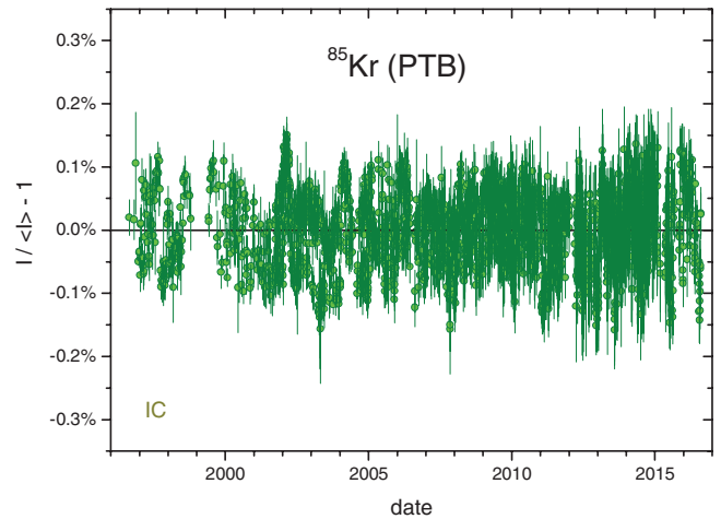
Figure 23. Residuals from exponential decay for ^{85}\text{Kr} ionisation current measurements (relative to the ^{226}\text{Ra} check source) with the IG12 IC at PTB, after applying linear detrending corrections.
