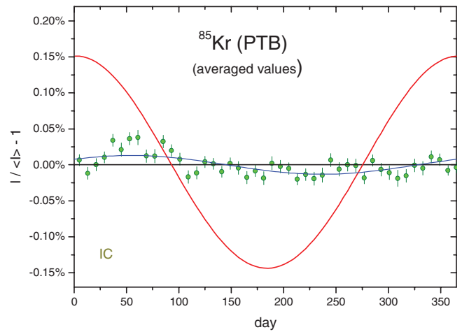
Figure 24. Annual average residuals from exponential decay for ^{85}\text{Kr} ionisation current measurements (relative to the ^{226}\text{Ra} check source) with the IG12 IC at PTB.
