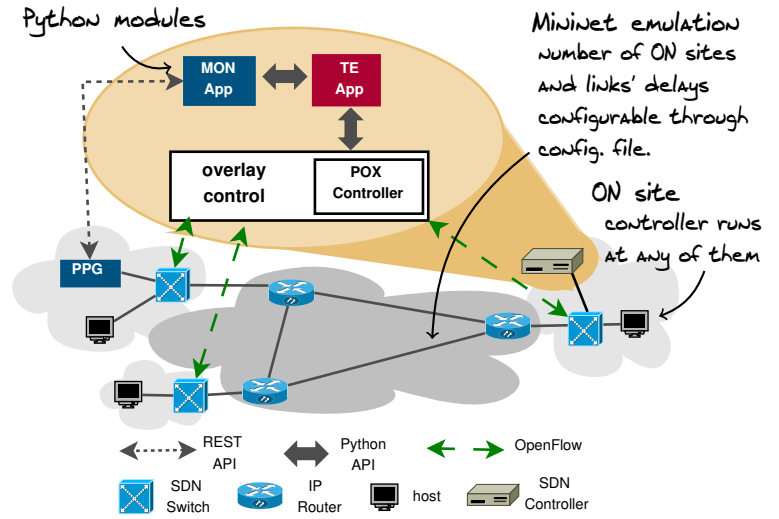
Fig. 2: Demonstration architecture
