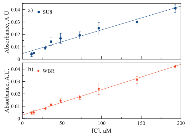
Fig. 5. Plots of absorbance versus concentration of fluorescein in DI water measured in PhLoCs fabricated using a) SU-8 and b) DuPont (WBR) master molds. Lines represent the least squares fitting of the experimental data.
