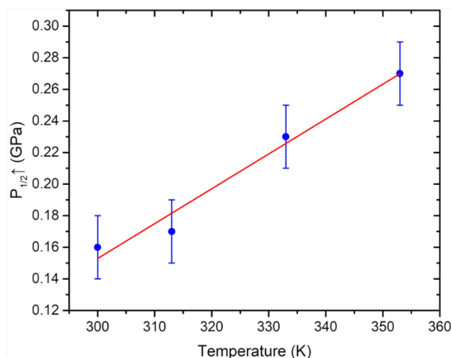
Figure 4. Variation of the pressure of SCO observed by increasing the pressure at a fixed temperature, P_{1/2} \uparrow , as a function of the temperature. The values of pressure are calculated from powder X-ray diffraction data Rietveld refinements of the HS and LS phases leading to the HS and LS fractions. P_{1/2} \uparrow corresponds to the pressure where HS and LS phases count for 50 % each.
