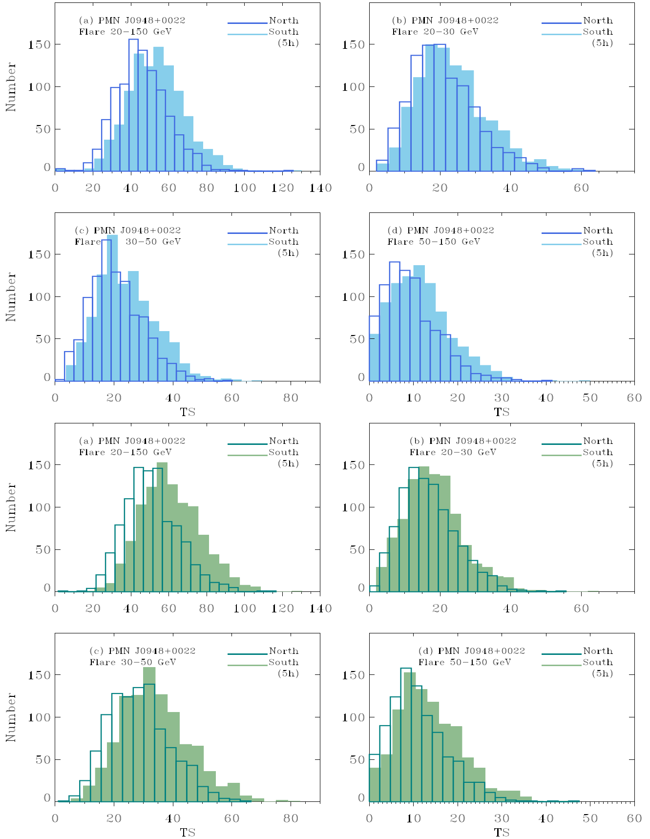
Figure A1. PMN J0948+0022 in ‘flare’ (exposure 5 h): comparison of distributions of the TS values depending on the energy band for detection. Blue: \text{edisp=no} , green: \text{edisp=yes} . See Table 3 and A1 for details.
