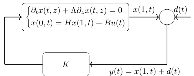
Fig. 1: Closed-loop system.
