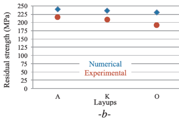
Fig. 5. Experimental/numerical comparison of permanent indentation (a) and residual strength (b) for A, K and O layups after 25 J impact.
