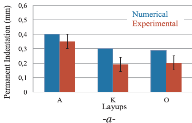
Fig. 5. Experimental/numerical comparison of permanent indentation (a) and residual strength (b) for A, K and O layups after 25 J impact.
