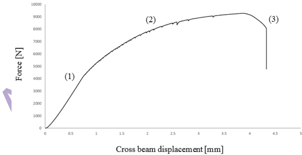
FIG. 9: Force-displacement of the chain
