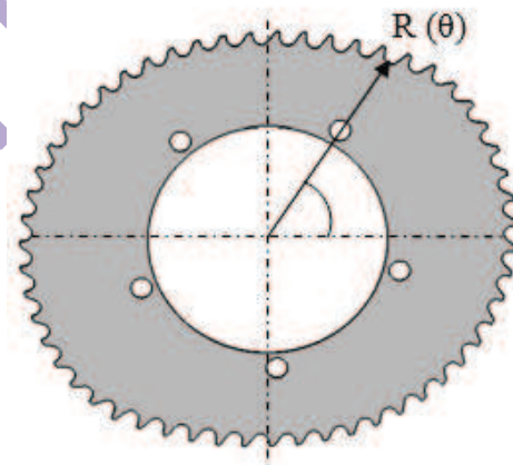
FIG. 2: Geometry of noncircular chainring
