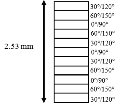
FIG. 6: Eleven plies stacking of noncircular composite chainring
