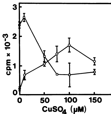
FIG. 3. Effect of \text{CuSO}_4 on ^{125}\text{I} -rANG specific binding. CPAEs (187,000 cells per 4\ \text{cm}^2 ) were incubated at 4^\circ\text{C} with ^{125}\text{I} -rANG (0.25 nM; 180,000 cpm) and increasing amounts of \text{CuSO}_4 as described in Fig. 2. \square , Washing buffer; \circ , solubilization buffer.
