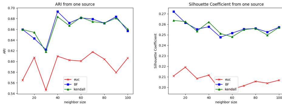
Fig. 3. ARI and silhouette coefficient, switch = 2
