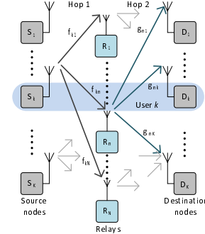
Fig. 1: Considered multi-user multi-relay network model.
