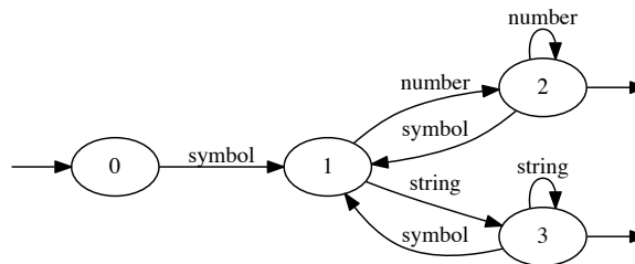
Fig. 3. Example DFA
