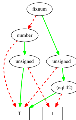
Fig. 6. Common Lisp type, (\text{or } (\text{not } \text{number}) (\text{eq } 42) (\text{and } \text{fixnum } (\text{not } \text{unsigned})) (\text{and } \text{unsigned } (\text{not } \text{fixnum}))) represented as ROBDD. The symbols \perp and \top refer to false and true respectively.
