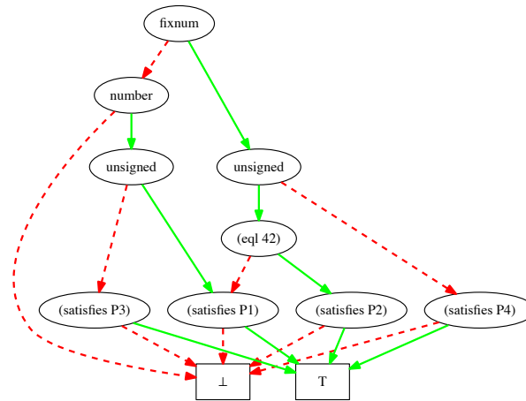
Fig. 9. ROBDD from typecase clauses in Example 7
