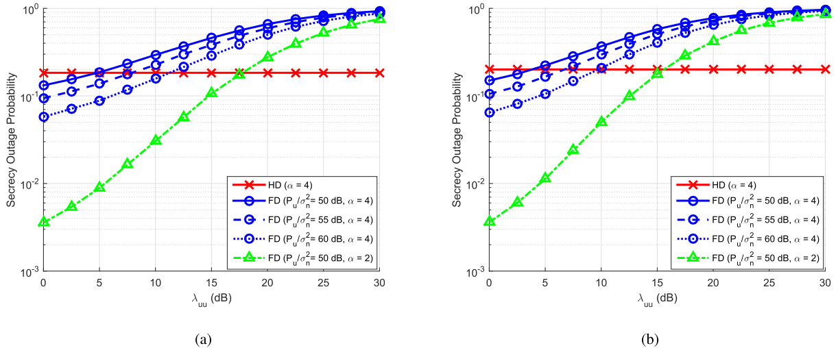
Fig. 6. The comparison of secrecy outage probabilities for FD and HD UEs with different residual self-interference channel gains, where d_{BU} = 10 m, R = 50 m and \rho_E = 0.001 m ^{-2} . (a) Independent EDs. (b) Colluding EDs.
