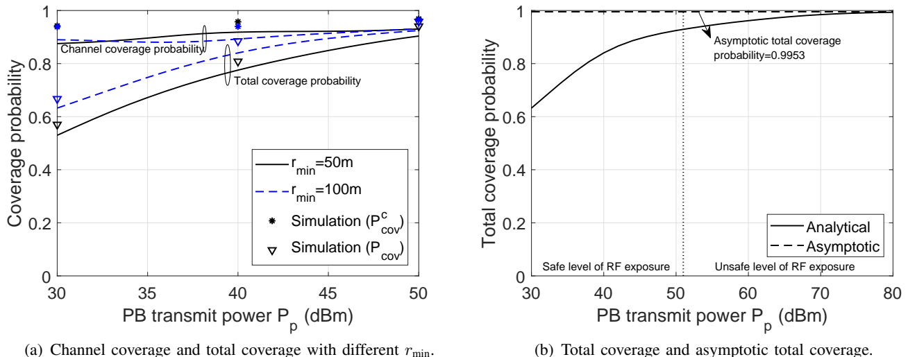
Fig. 4: Coverage probabilities versus PB transmit power P_p .
