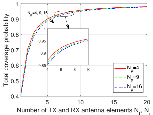
Fig. 6: Total coverage probability versus the numbers of antenna elements at TX and RX \mathcal{N}_t and \mathcal{N}_r with different numbers of antenna elements at PB.
