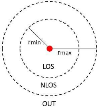
Fig. 1: Illustration of mmWave blockage model.
