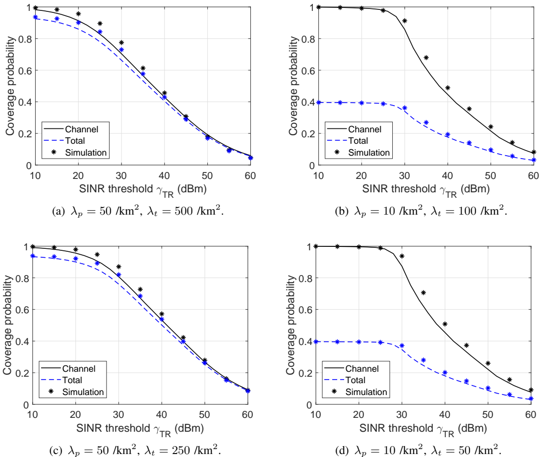
Fig. 3: Channel coverage probability and total coverage probability versus SINR threshold \gamma_{TR} . The PB density is 50 and 10 per \text{km}^2 and the TX density is 500, 100, 250 and 50 per \text{km}^2 .
