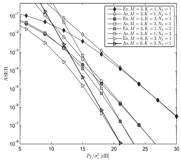
Fig. 9. ASER vs. asymptotic ASER for several system setups. When K = 1 , the ASER corresponds to the CP-SC system with selection combining.
