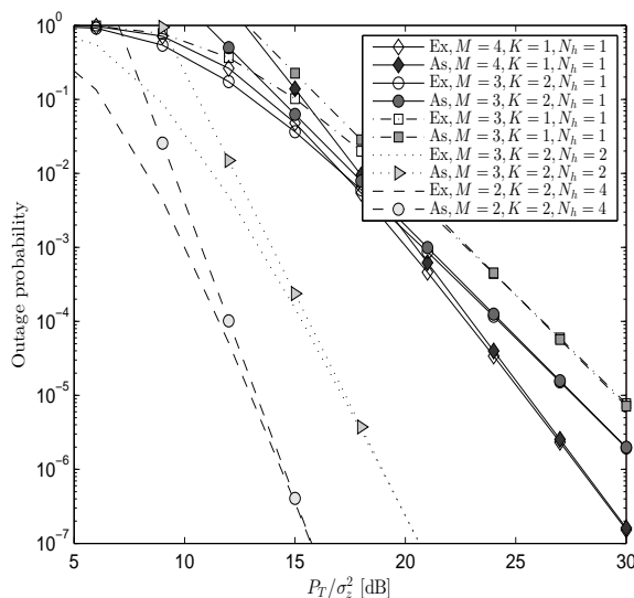
Fig. 8. Outage probability vs. asymptotic outage probability for several system setups. When K = 1 , the outage probability corresponds to the CP-SC system with selection combining.
