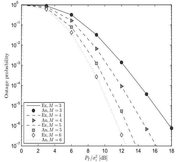
Fig. 3. Outage probability for several system setups.
