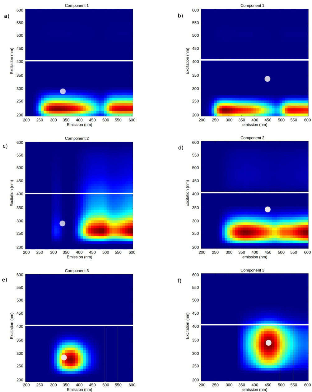
Figure 2: Components C1_T , C2_T and C3_T (figure a, c, e) of \{\text{TRP-HA-BA}\} system (left), and component C1_B , C2_B and C3_B (figure b, d, f) of \{\text{QS-BA}\};\{\text{QS-HA}\} systems (right). The white line represents the 405 nm laser induced fluorescence excitation wavelength and the white circle represents the maximum fluorescence peak position of the TRP (left column) and of the QS (right column) in solution.
