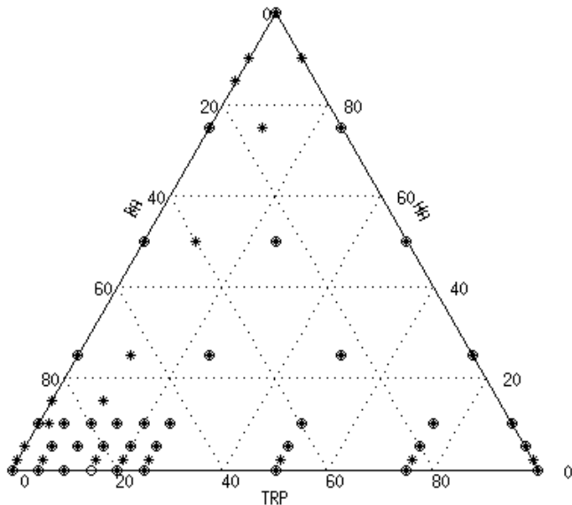
Figure 1: Experiment plan of samples preparation for the {TRP-BA-HA} ternary system. Stars (*) represent ten measurements at different angles and faces, and circle (o) single two face measurement. Each side of the triangle represents the variation from 0 to 100% of the labeled molecule in the ternary system (down side the Tryptophan (TRP), right side the Boric Acid (BA), and left side the Humic Acid (HA)).
