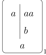
Figure 3: The P system \Pi_3 with randomized pools of RHS generating the number language \{2^n \mid n \in \mathbb{N}\} .
