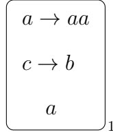
Figure 2: The P system \Pi_2 with random RHS exchange generating the number language \{2^n \mid n \in \mathbb{N}\} .
