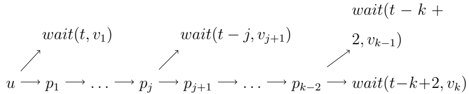
Figure 8: Timers allow sequential choice between any number of right-hand sides.
