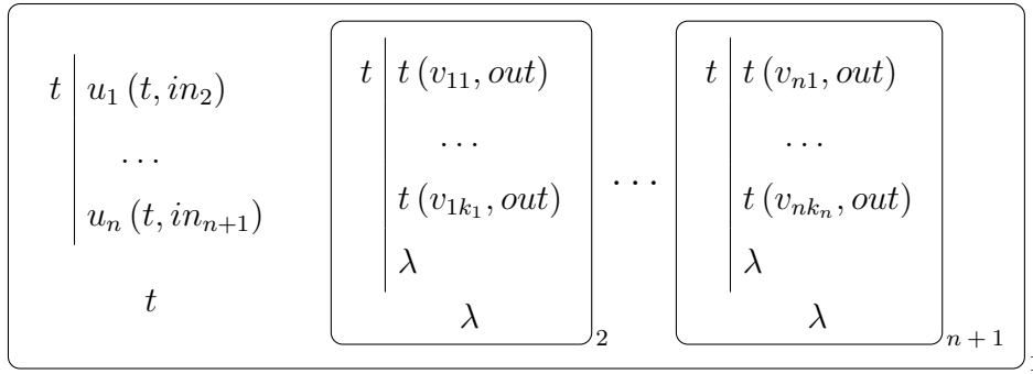
Figure 6: The P system \Pi_6 with randomized pools of RHS generating the semilinear language L = \bigcup_{1 \leq i \leq n} \langle A_i, \mathbf{b}_i \rangle_{\mathbb{N}} .
