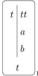
Figure 7: The P system \Pi_7 with randomized pools of RHS generating the union language L'_{ab} = \{a^{2^n} \mid n \in \mathbb{N}\} \cup \{b^{2^n} \mid n \in \mathbb{N}\}
