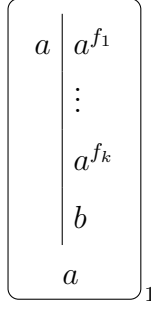
Figure 5: The P system \Pi_5 with randomized pools of RHS generating the number language \{f_1^{n_1} \dots f_k^{n_k} \mid n_1, \dots, n_k \in \mathbb{N}\} .
