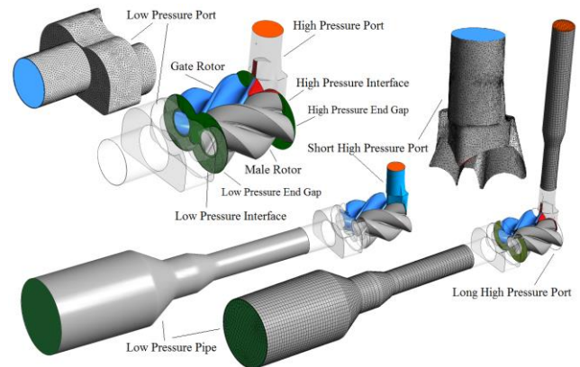
Figure 2. Typical representative of a numerical mesh for CFD calculation of screw compressors
