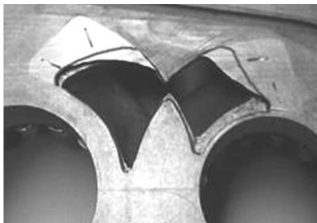
Figure 12 Influence of the port shape on noise generation
