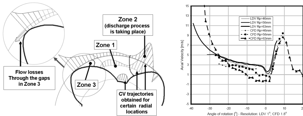
Figure 6 Flow zones identified in the results (left) and comparison of the LDV and CFD axial velocities
