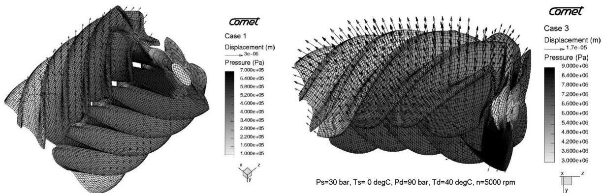
Figure 7 Oil injected screw compressor for moderate pressures (left) and high discharge pressures (right)
