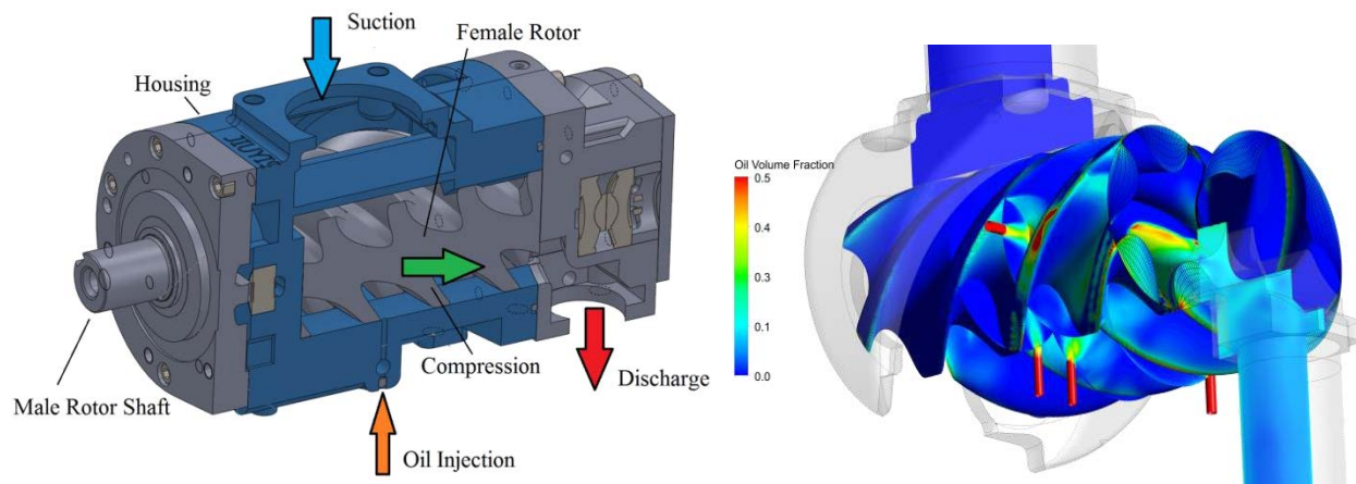
Figure 16 Oil injected screw compressor (left) and CFD simulation of oil distribution (right)
