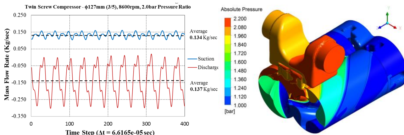
Figure 3 Mass flow rate variations in the ports (left) and contours of pressure variation (right)
