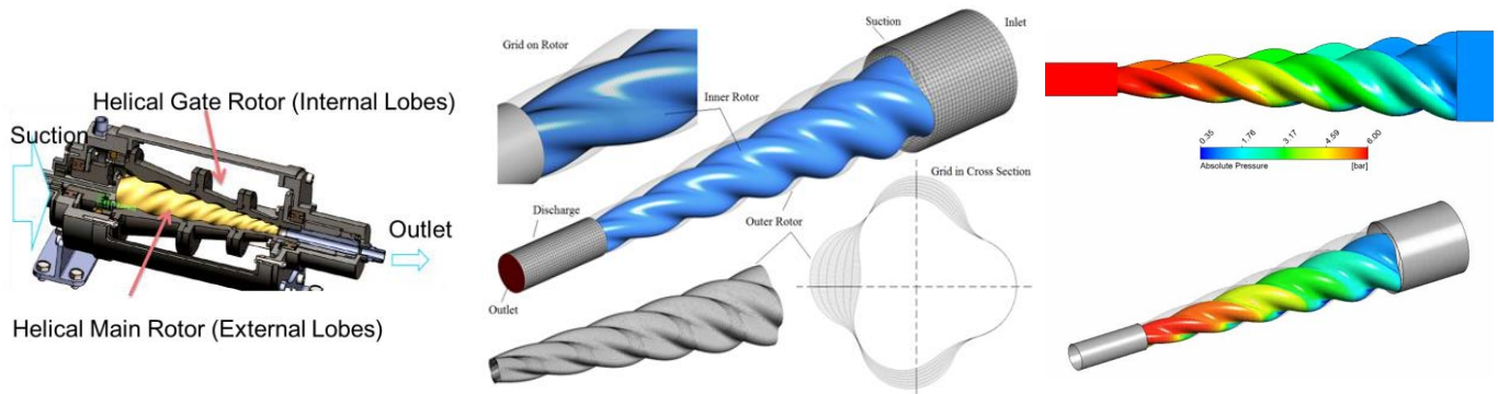
Figure 15 Conical internally geared screw compressor, numerical mesh and pressure on the rotor surface
