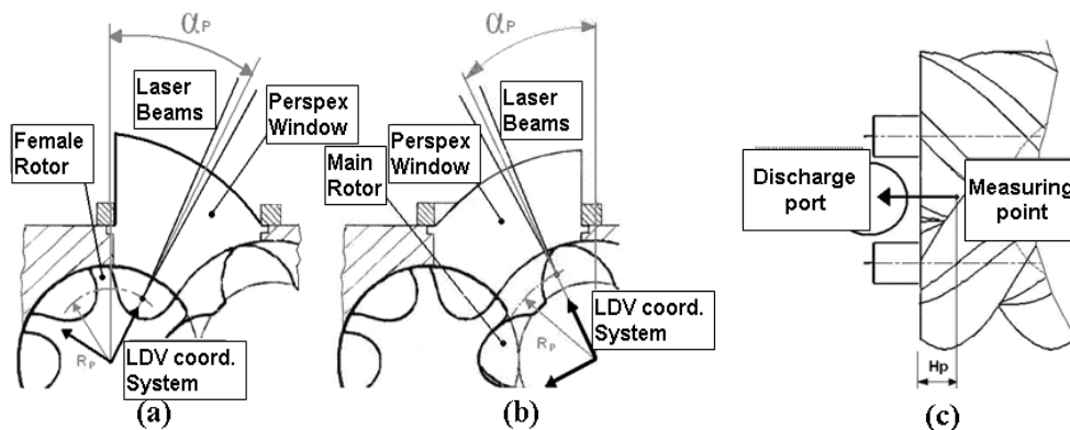
Figure 5 Position of coordinate systems and optical access windows the female (a) and male rotor (b); axial position (c)
