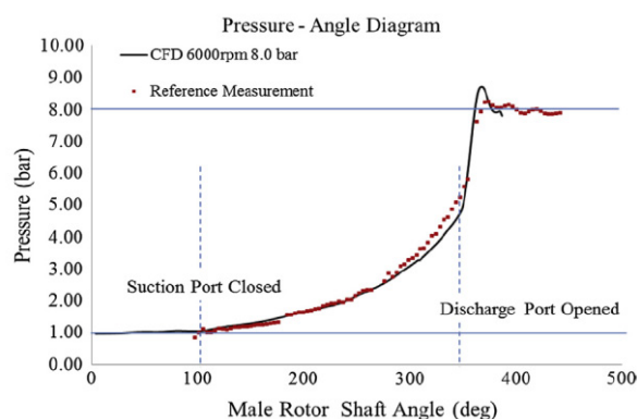
Figure 17 Comparison of experimental and measured results
