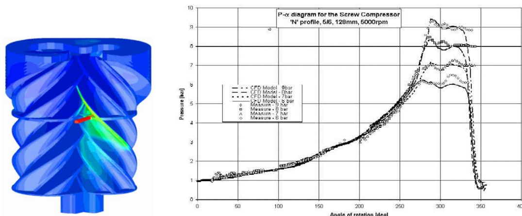
Figure 4 Oil injection and Comparison of measured and calculated pressures
