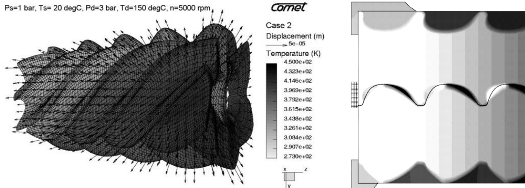
Figure 8 Rotor displacement vectors and temperature distribution for an oil free compressor
