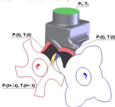
Figure 9 3D domain of the screw compressor discharge chamber and full 3D model showing the interface
