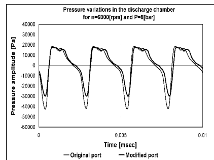
Figure 12 Influence of the port shape on noise generation
