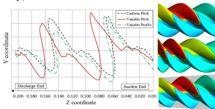
Figure 14 Comparison of interlobe sealing line lengths for constant and variable rotor geometry compressor
