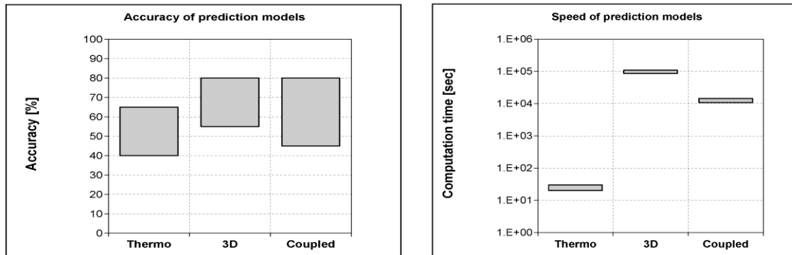
Figure 11 Accuracy and speed of numerical models
