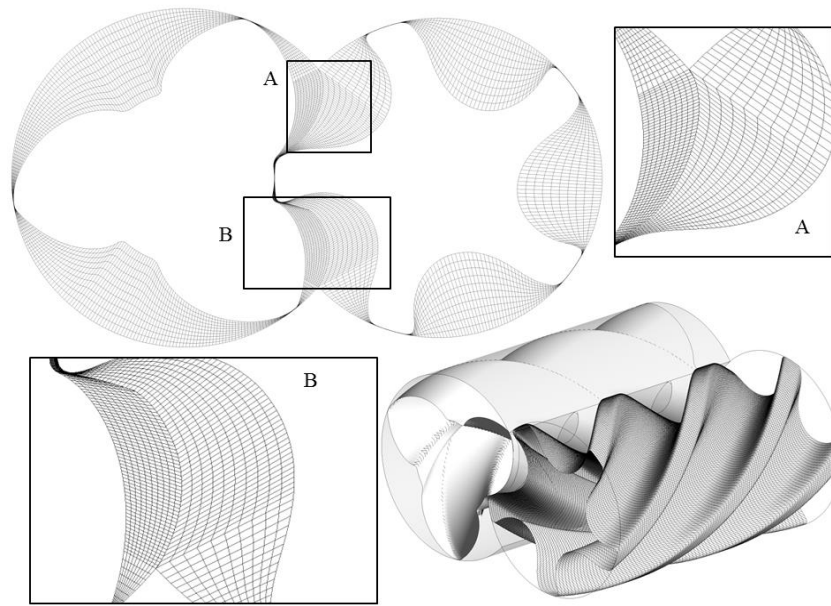
Figure 13 Numerical mesh generated using rotor-to-rack boundary distribution and background blocking
